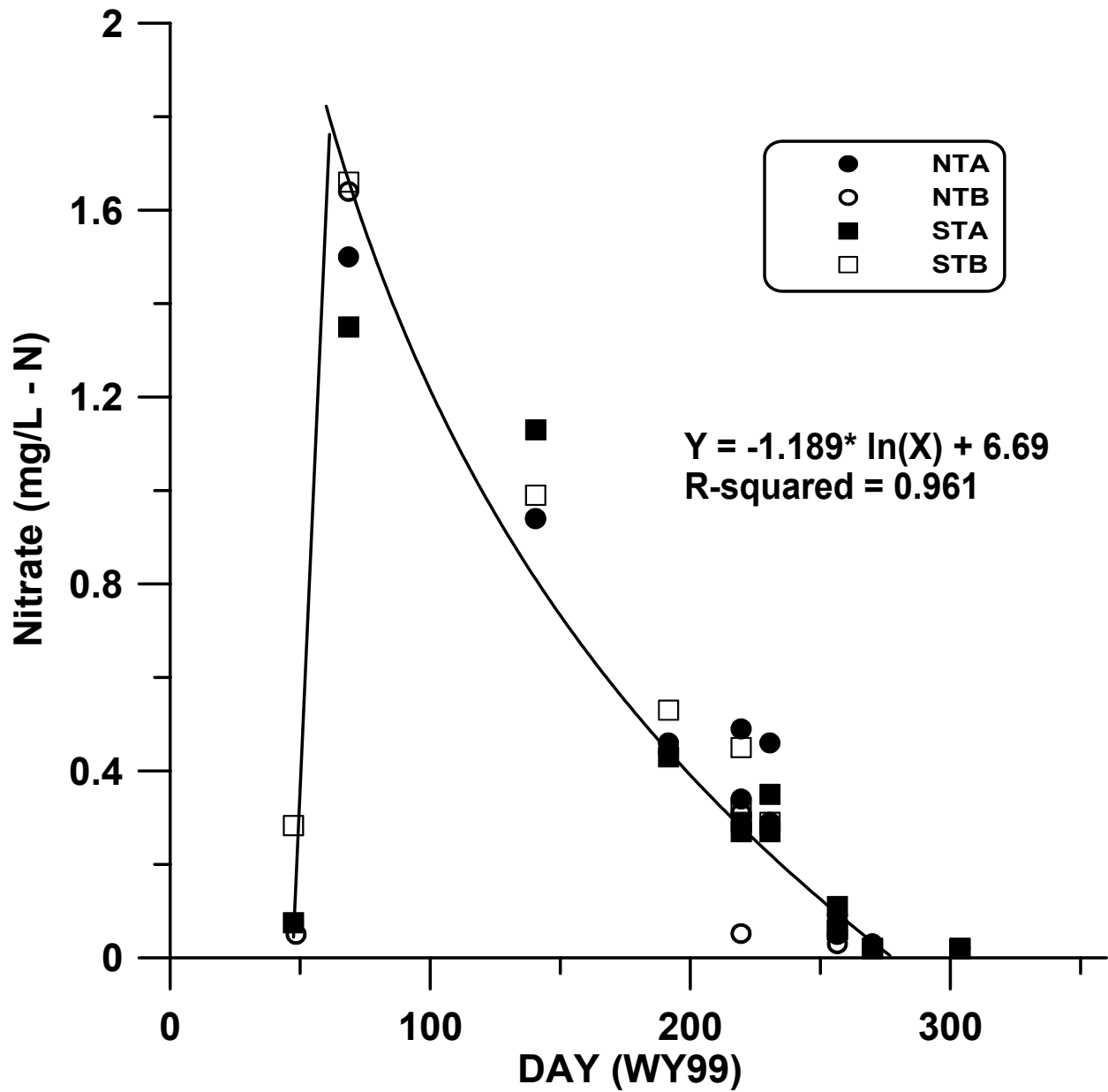
Figure 26. Concentration of nitrate (NO 3 -N, mg/L) versus Julian day for the four lake sites.
