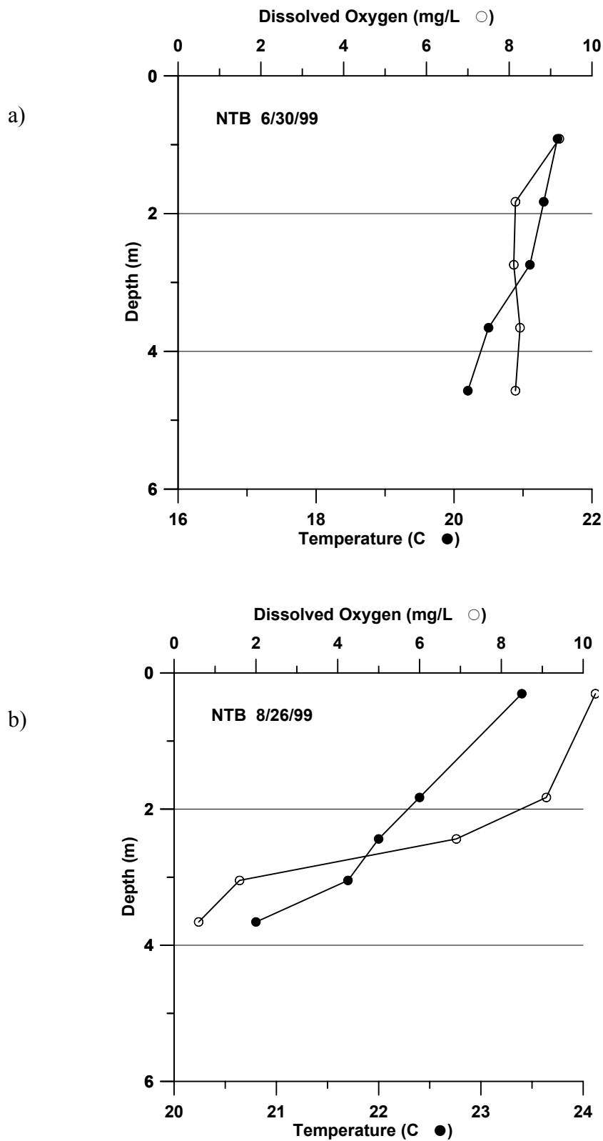
Figure 18. Temperature (°C) and dissolved oxygen (mg/L) at NTB (North Tenmile-Site B) versus depth (m) on a) June 30, 1999 and b) August 26, 1999.
