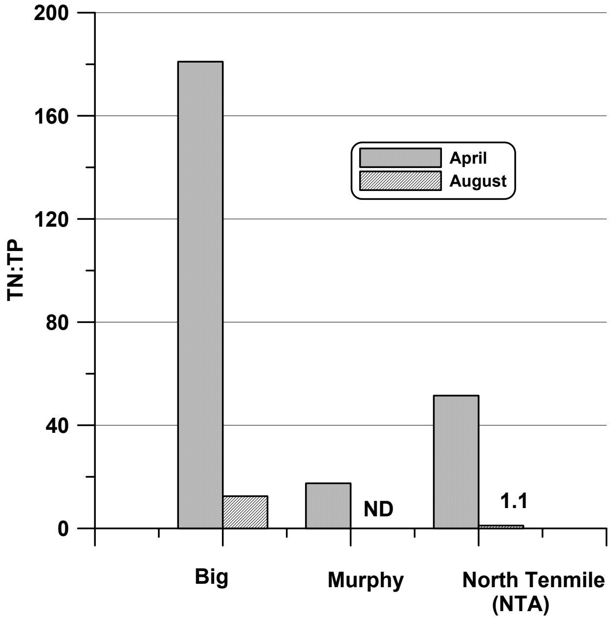
Figure 36. Ratio of total nitrogen to total phosphorus (TN:TP) for selected tributary and lake sites for the months of April and August.
