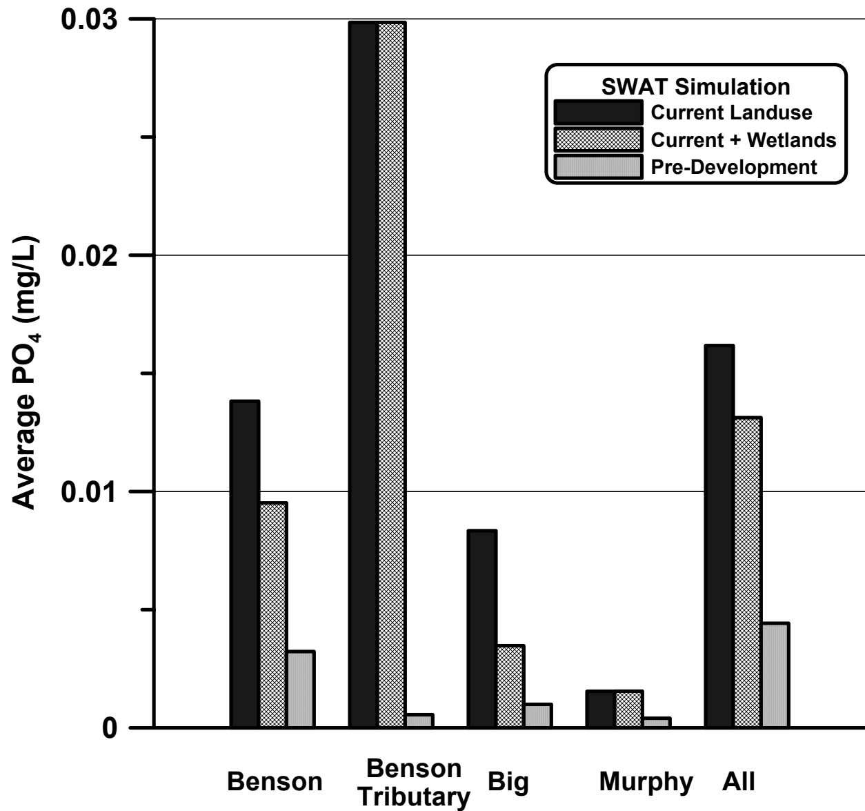
Figure 61. SWAT model simulations of phosphorus export (as flow-weighted concentrations) for monitored stream sites.
