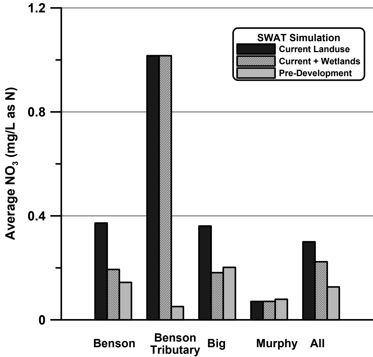
Figure 62. SWAT model simulations of nitrate export (as flow-weighted concentrations) for monitored stream sites.
