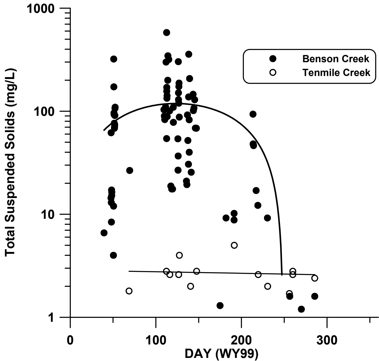
Figure 23. Total suspended solids (TSS, mg/L) versus Julian day for Benson Creek (●) and the outlet of Tenmile Creek (○). The lines represent the best fits for Benson Creek (power function) and Tenmile Creek (linear function).
