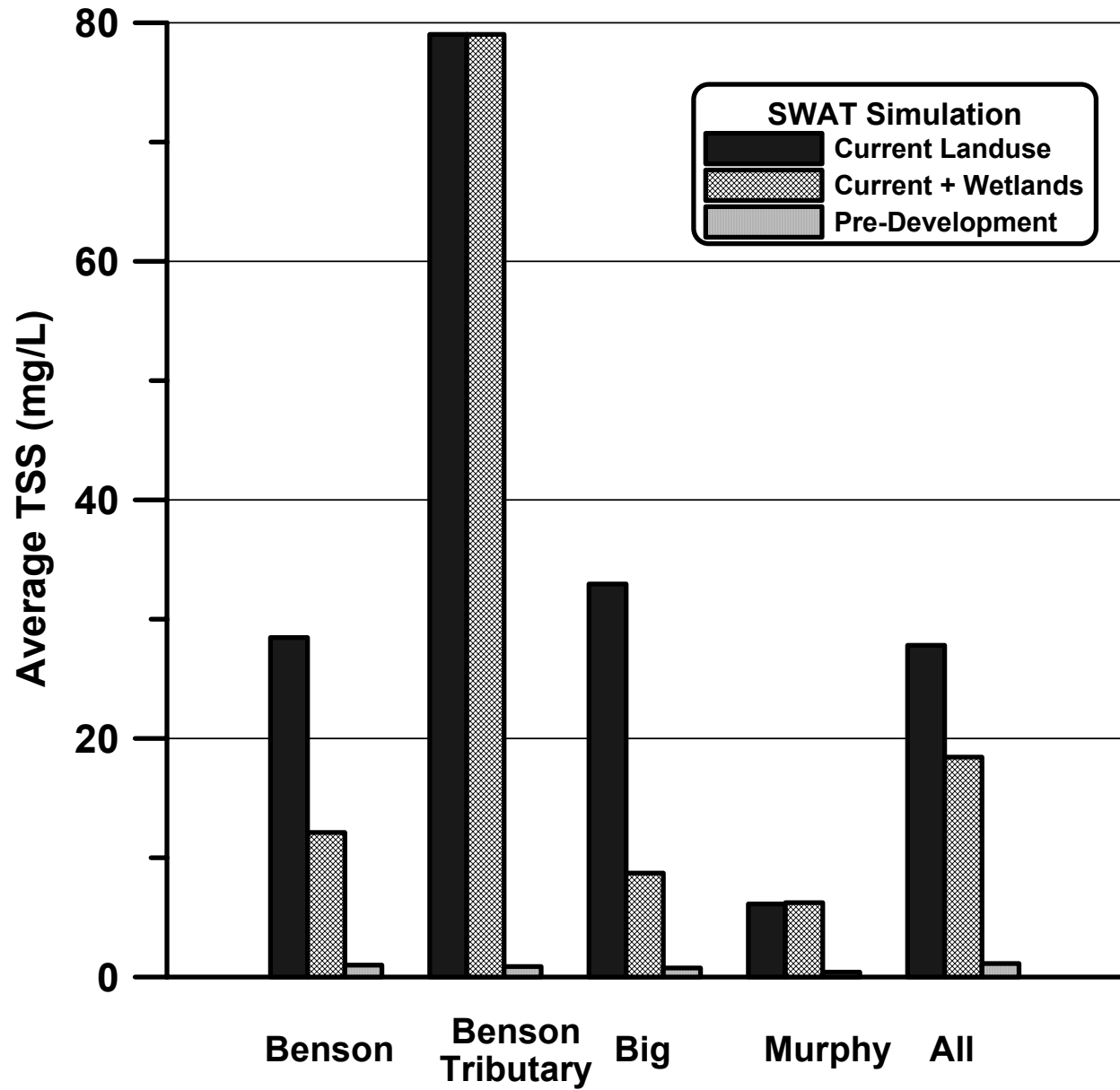
Figure 60. SWAT model simulations of sediment export (as flow-weighted concentrations) for monitored stream sites.
