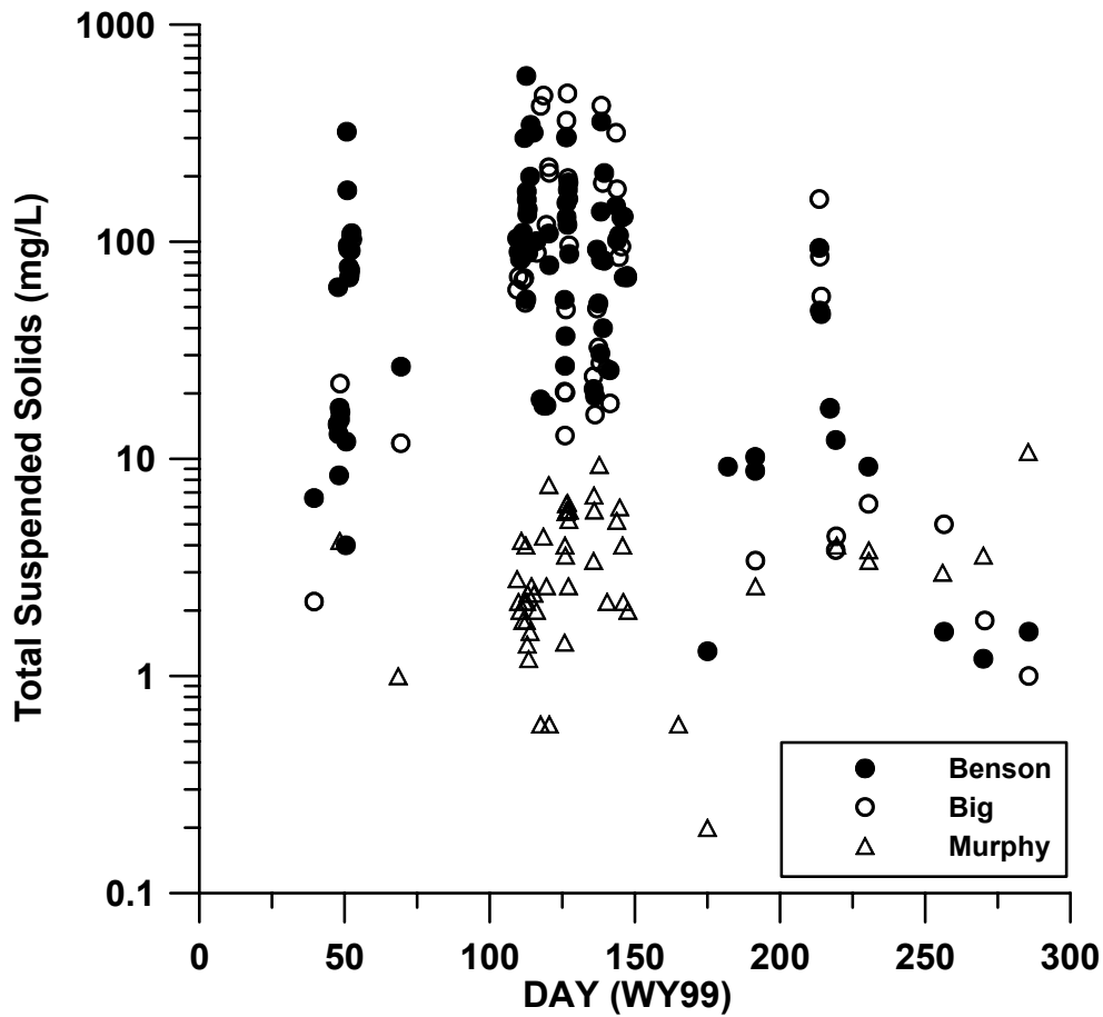
Figure 10. Total suspended solids (TSS, mg/L) for Big, Benson, and Murphy Creeks, WY1999. Note that the data are presented on a log 10 scale.
