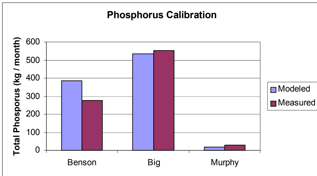
Figure 54. Simulated versus measured concentrations of TP (mg/L) for Big, Benson, and Murphy Creeks.
