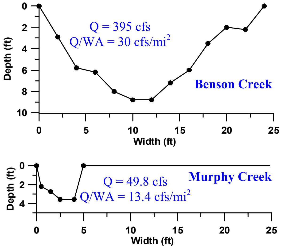
Figure 70. Stream channel cross sections for Benson Creek (top) and Murphy Creek (bottom) at the water quality monitoring sites. The stream discharge (Q, cfs) and discharge normalized per unit area (Q/WA, cfs/mi 2 ) is shown for both sites at bank-full flows.
