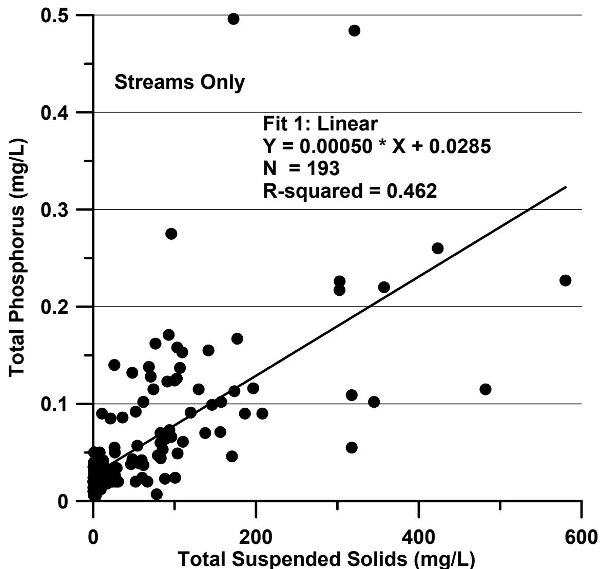
Figure 65. Relationship between total phosphorus and total suspended solids for tributaries to Tennile Lake.
