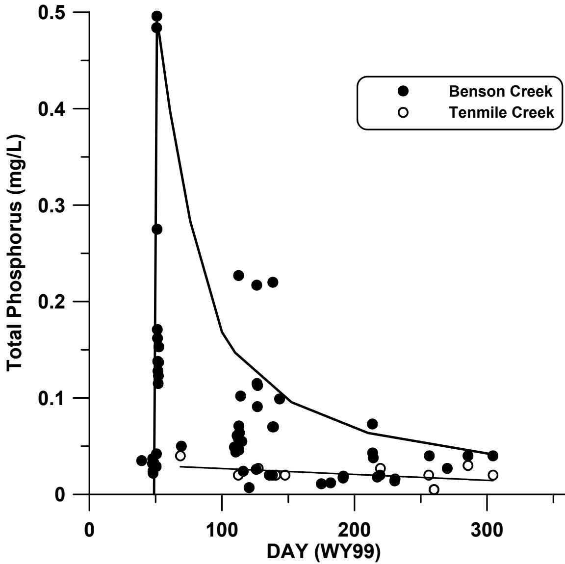
Figure 25. Concentrations of total phosphorus (TP; mg/L) versus Julian Day for Benson Creek (●) and Tenmile Creek (○).
