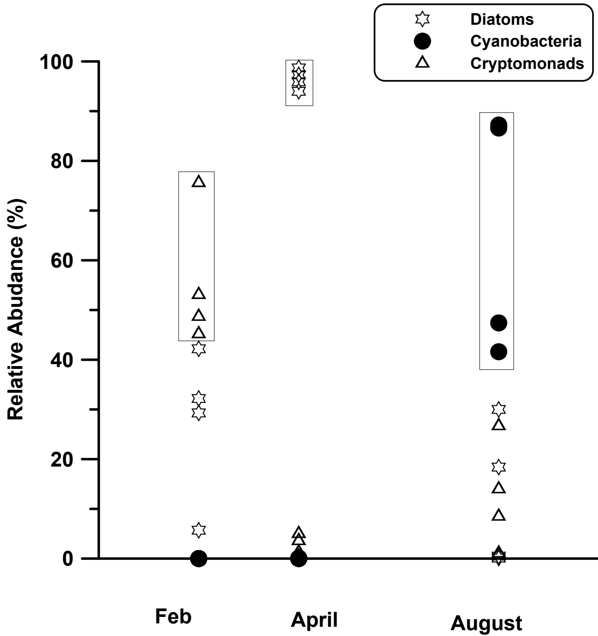
Figure 34. Relative abundance (based on present biovolume) of major taxa of phytoplankton in Tennile Lake as a function of season.
