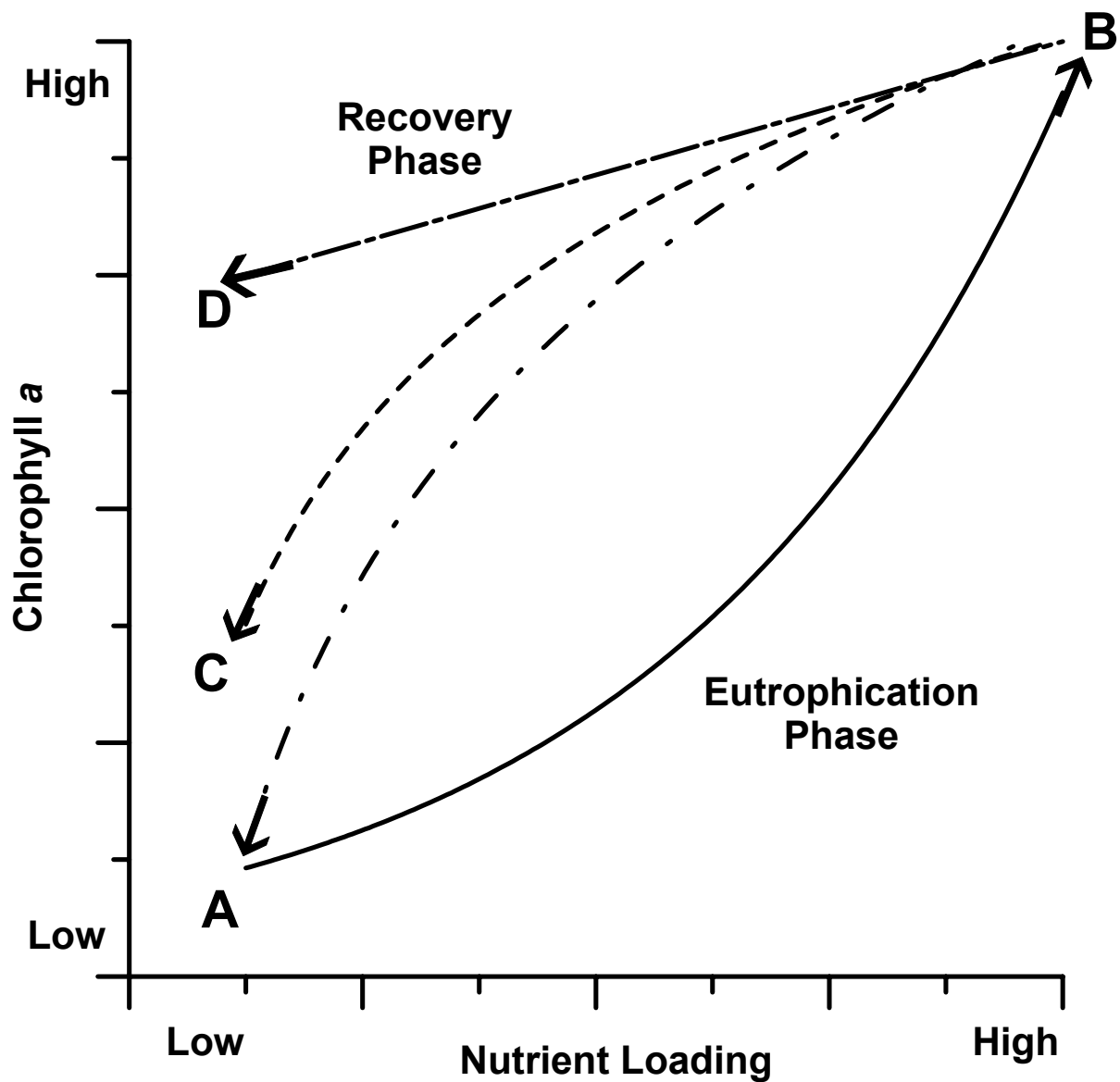
Figure 69. A schematic representation of lake response to increased nutrient loading (curve A → B) and multiple scenarios for lake response to decreased nutrient loading (B → A; B → C; and B → D) depending on factors within the lake.
