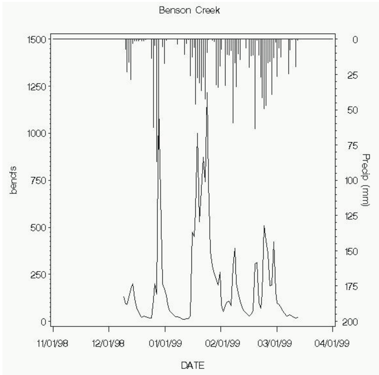
Figure 6. Stream discharge in Benson Creek (cfs) and precipitation collected on-site.
